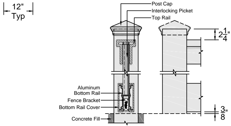
Post Profile: Cut View / Elevation View
