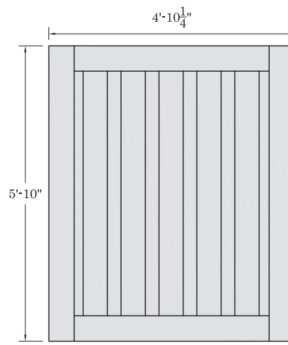
STANDARD 10' X 6' DOUBLE GATE PANEL
