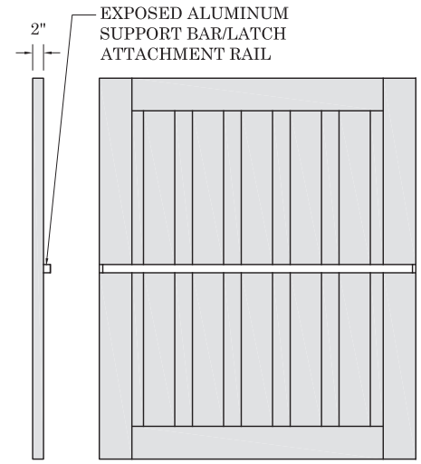
STANDARD 10' X 6' DOUBLE GATE PANEL
