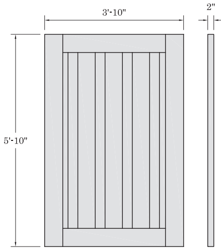
STANDARD 4' X 6' WALK GATE PANEL
